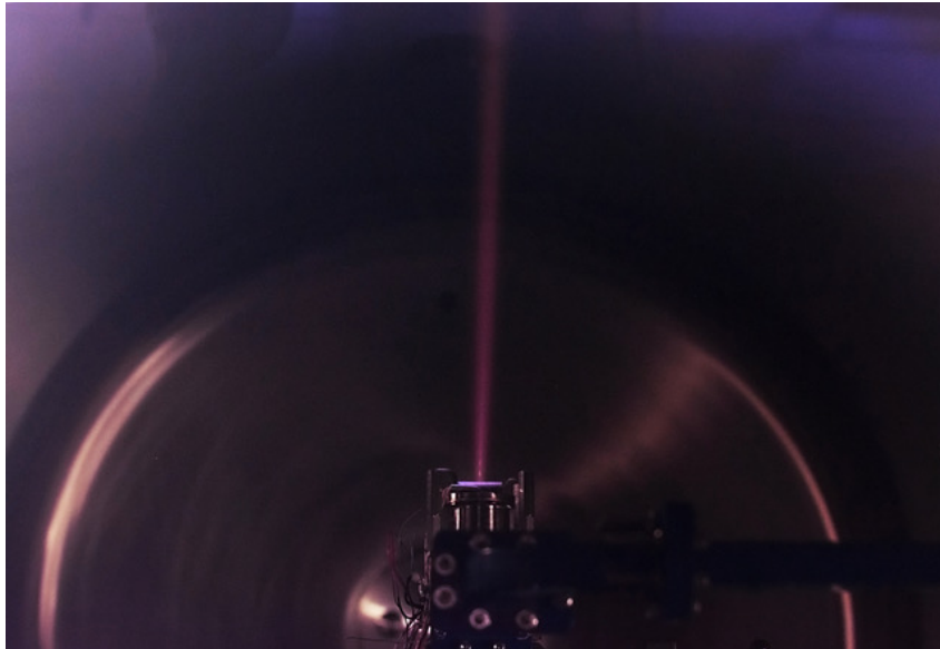
Momentus' latest-generation thruster undergoes testing in a vacuum chamber at company headquarters.
